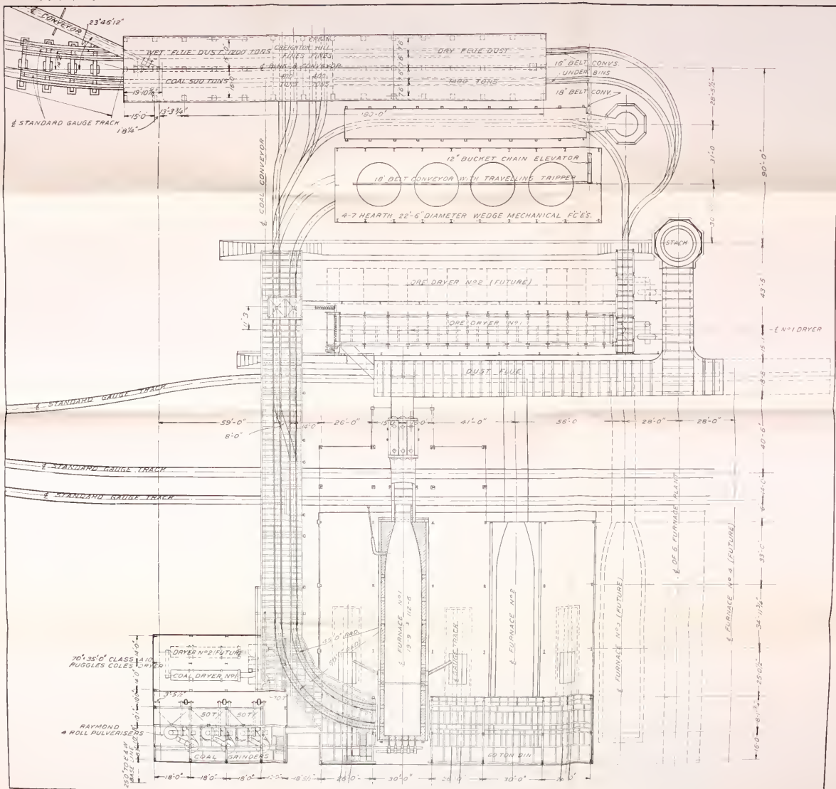
Plan and Lay-out of Reverberatory Department, 1915, Canadian Copper Company, Copper Cliff, Ontario
